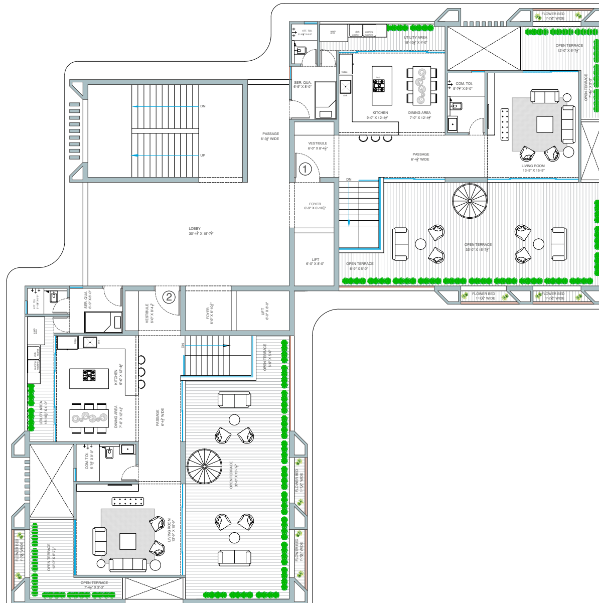
4.5 BHK Plan Tower C / Cluster Plan (12th Floor Plan - Penthouse Upper Level)
