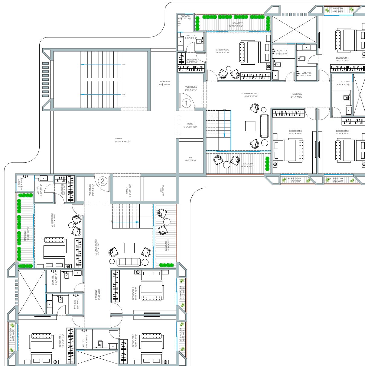
4.5 BHK Plan Tower C / Cluster Plan (11th Floor Plan - Penthouse Lower Level)
